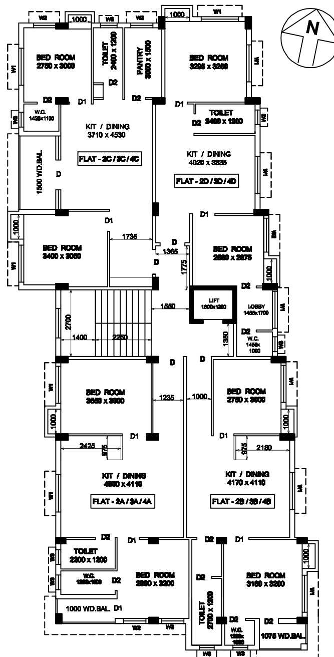
2ND,3RD & 4TH. FLOOR PLAN
